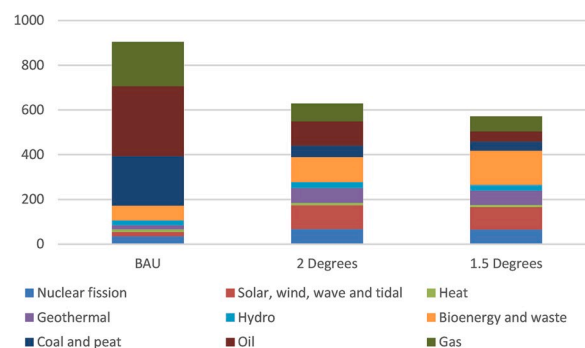
Fig. 4. Global energy supply in EJ (exa-Joules) by different GHG mitigation scenarios in 2050. Note: Approximate share of renewable energies in total primary energy supply for each simulation pathway in 2050: BAU, 14% out of 905 EJ in total; 2D, 49% out of 628 EJ in total; and 1.5D, 60% out of 572 EJ. Source: Prepared by the authors, using the Global Calculator.
