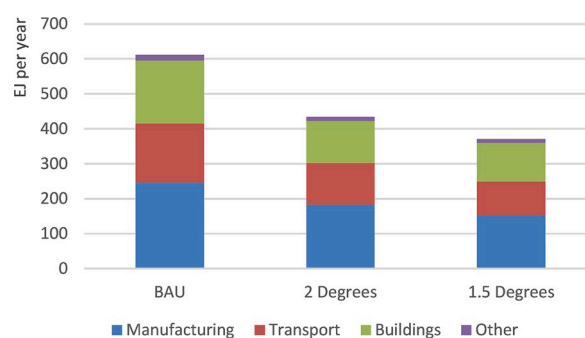
Fig. 3. Energy demand in EJ (exa-Joules) by different GHG mitigation scenarios in 2050. Source: Prepared by the authors, using the Global Calculator.
